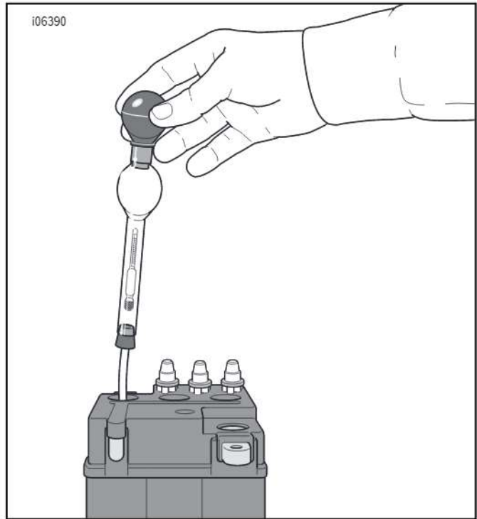
Figure 4. Hydrometer
