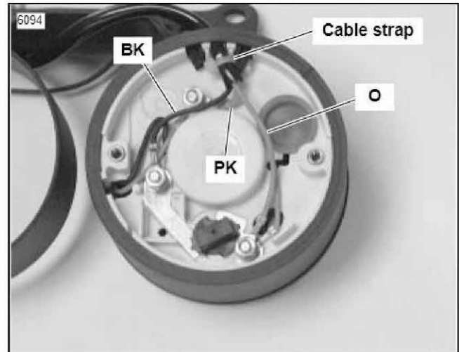
Figure 1. Tachometer Wiring
