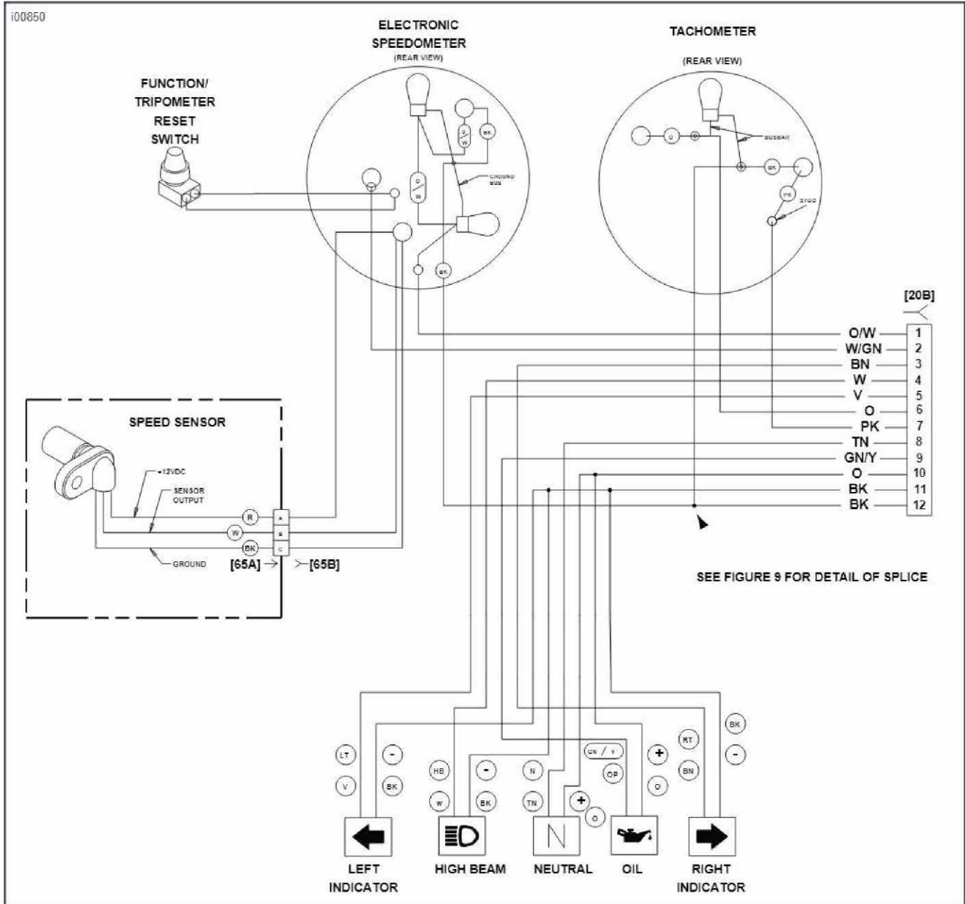
Figure 9. Wiring Schematic
