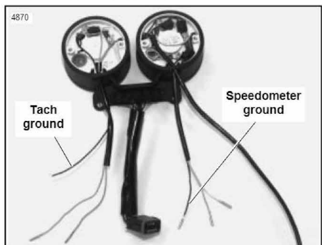
Figure 6. Speedometer in Double Bracket
