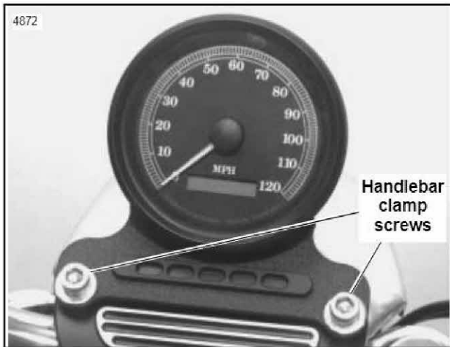
Figure 3. Removing Speedometer and Bracket
