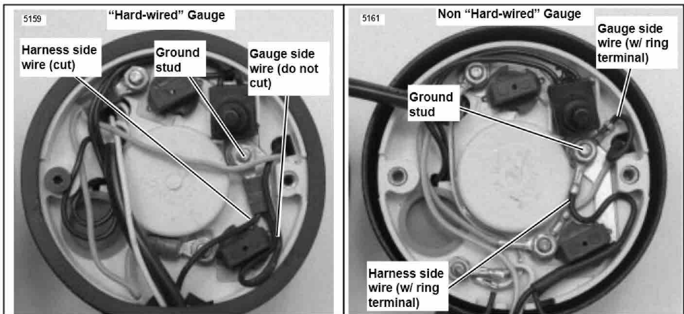
Figure 3. Gauges Comparison
