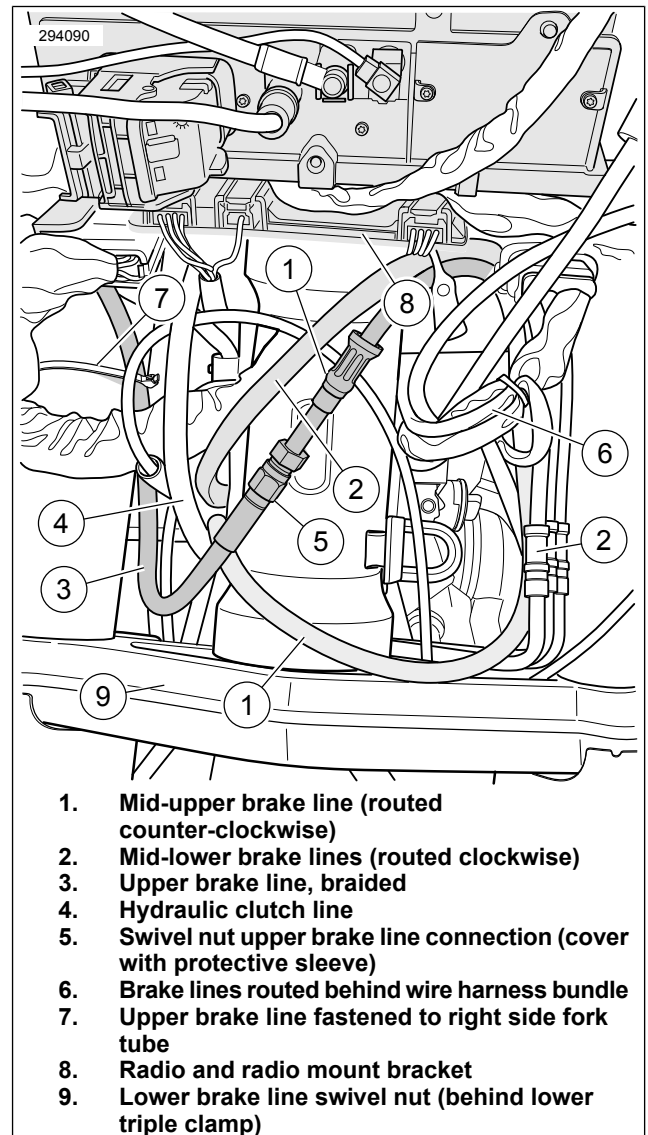
Figure 1. Outer Fairing View - Brake Line Routing: FLHT, FLHX
