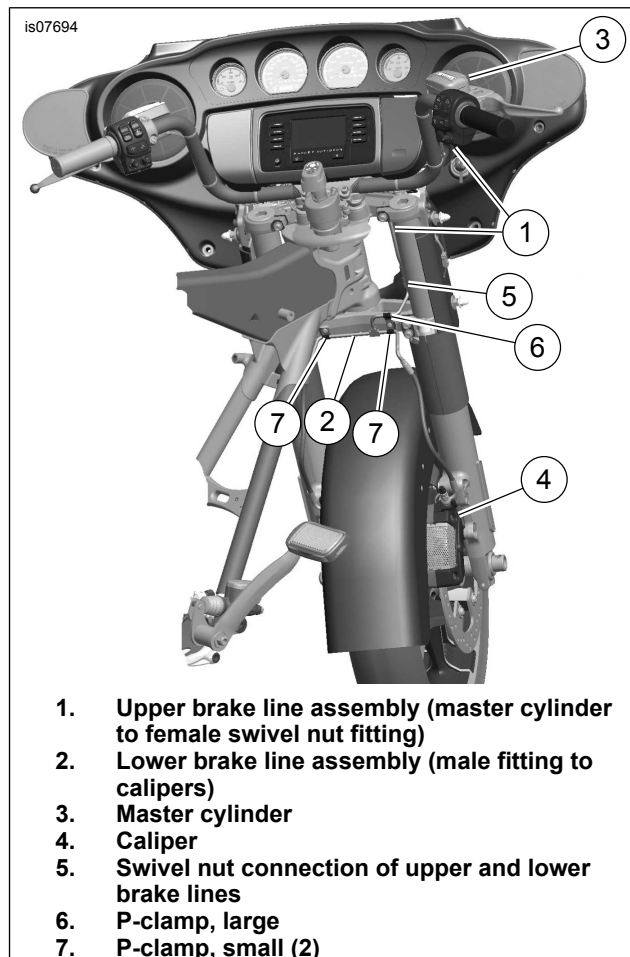
Figure 3. 2014 and later Front Non-ABS Brake Lines
