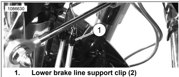
Figure 4. Lower Brake Line Support Clips
