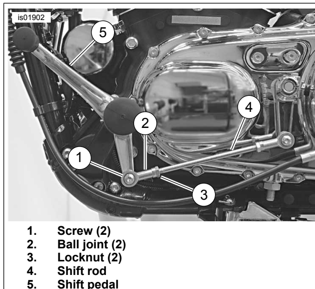
Figure 1. Adjusting Shift Pedal
