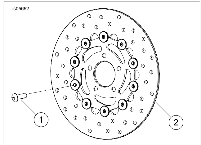
Figure 1. Service Parts: Reaper Floating Rotor Kits
