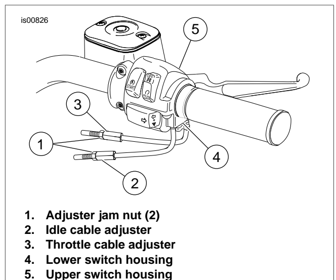
Figure 8. Handlebar Throttle Control
