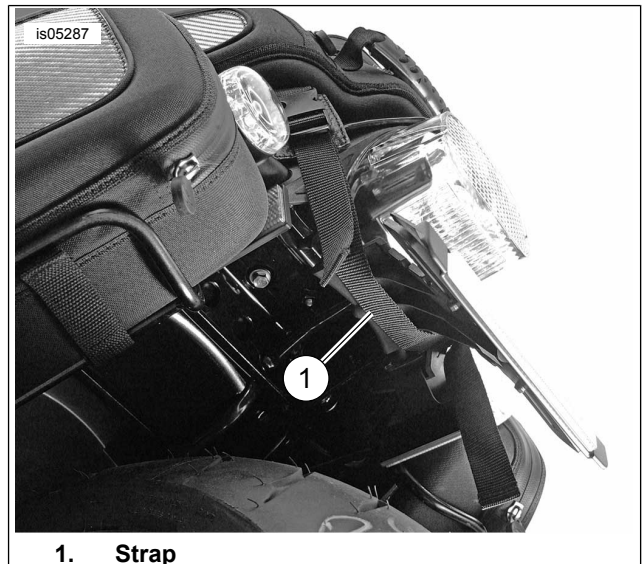
Figure 3. Tail Bag Rear Strap (shown with optional saddlebags)
