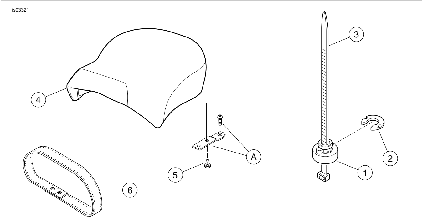
Figure 6. Service Parts: XL PASSENGER PILLION KIT
