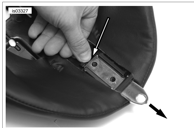
Figure 1. Seat Bracket Removal
