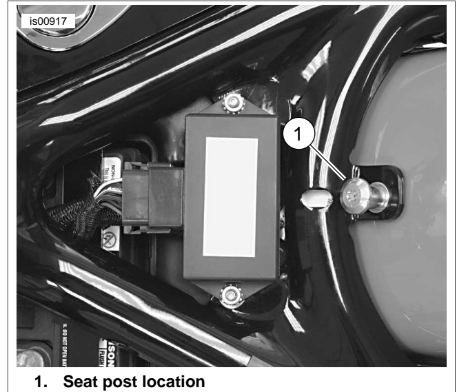
Figure 5. Seat Post
