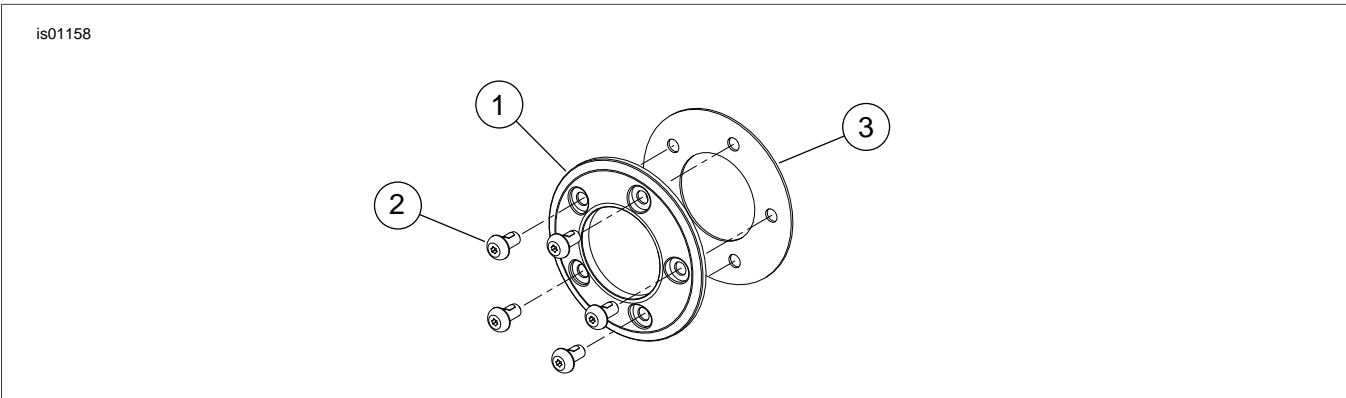
Figure 1. Service Parts: Front Wheel Hub Plate Kits
