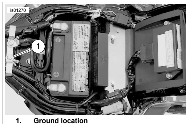
Figure 7. 2004 Softail Ground
