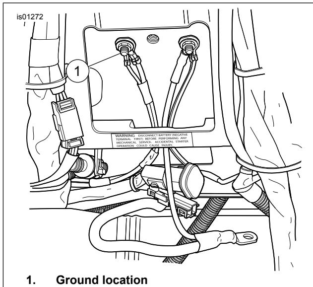
Figure 9. 2004 FLHR Ground
