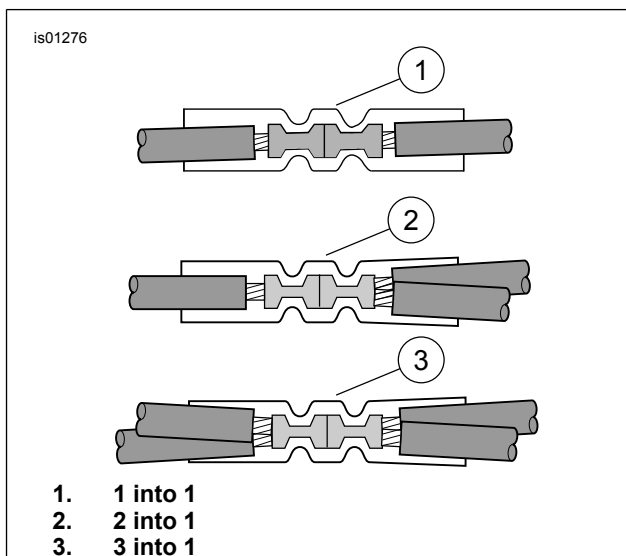
Figure 13. Splice Configurations
