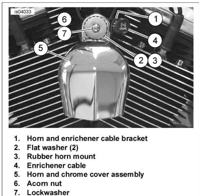
Figure 8. Horn Assembly Installation, 2004-2006 Models
