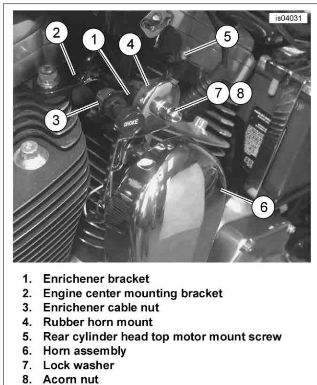
Figure 6. Horn Assembly Installation, 1995-2003 Models
