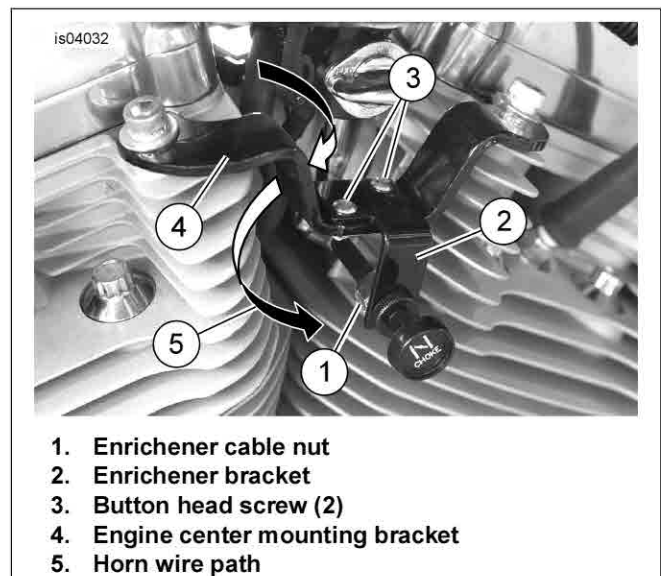
Figure 7. Original Enrichener Bracket, 2004-2006 Models
