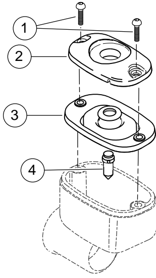
Figure 1. Service Parts: Brake Fluid Reservoir
