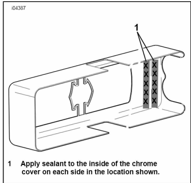
Figure 1. Inside view of Chrome Cover and Sealant Application
