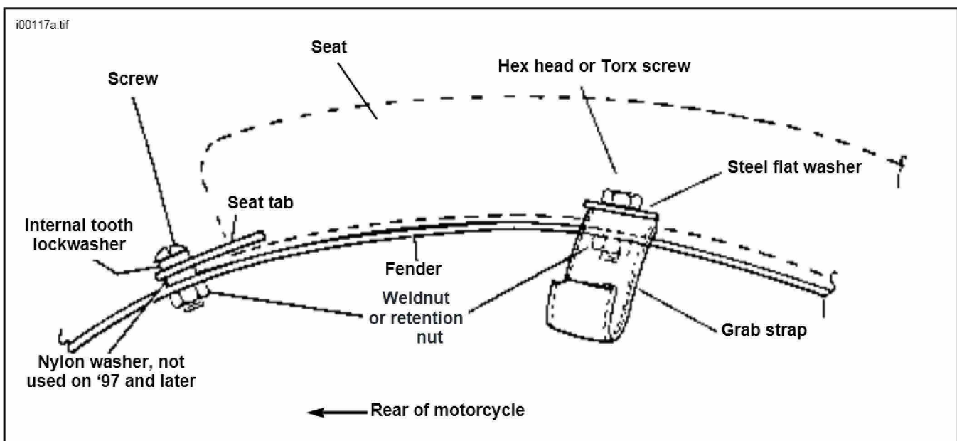
Figure 1. Hardware, Seat Bracket and Grab Strap Assembly
