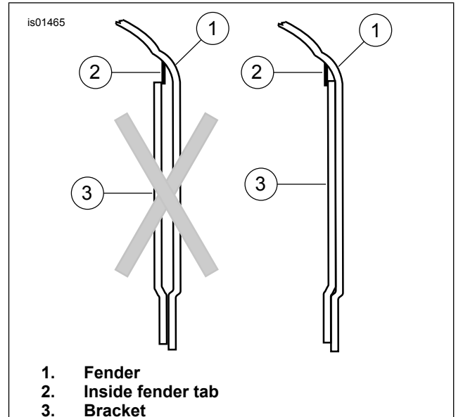
Figure 1. Position Inside Fender Brackets
