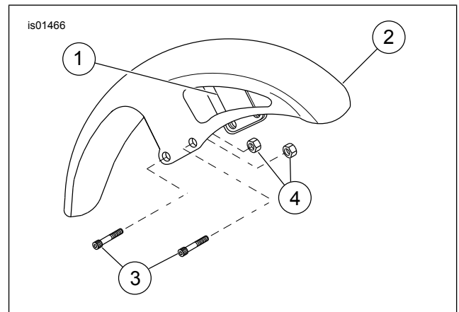
Figure 2. Service Parts: Front Fender
