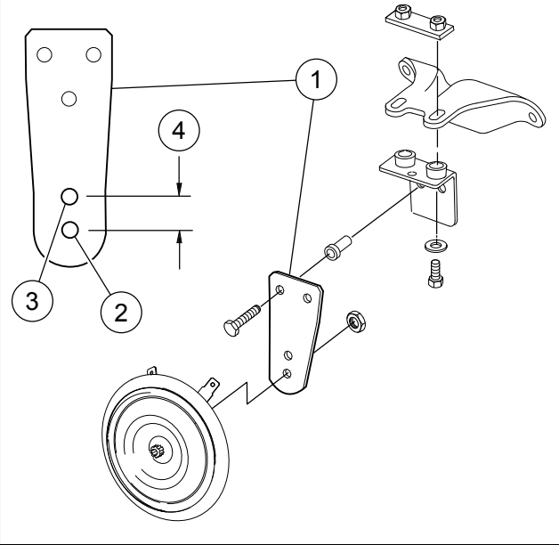
Figure 2. Relocating Horn 1/2 Inch Higher
