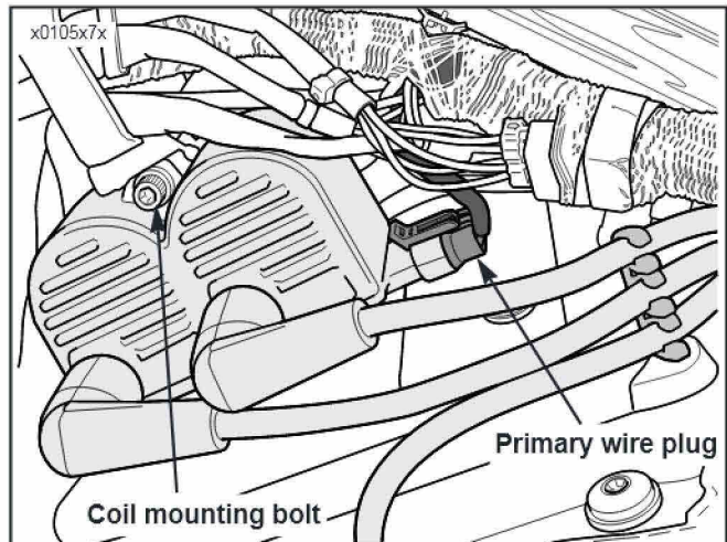
XL1200S Coil
