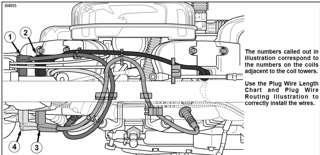
Spark Plug Wire Routing
