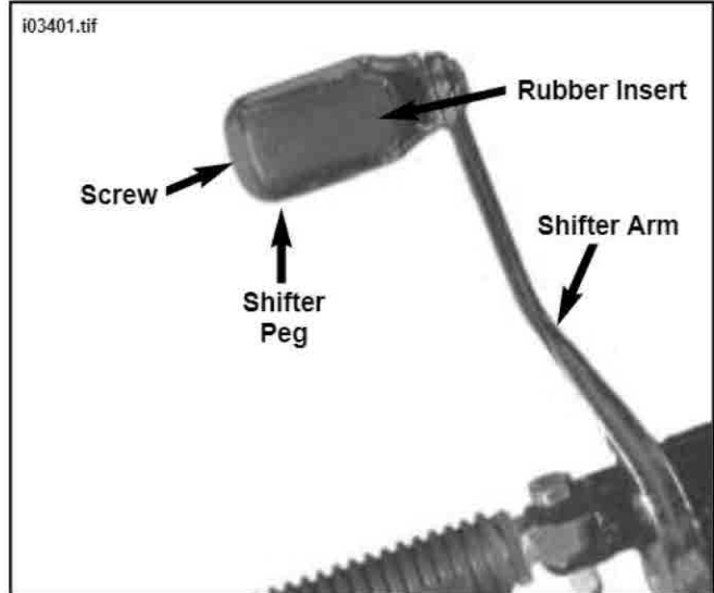
Figure 1. Shifter Peg Installation
