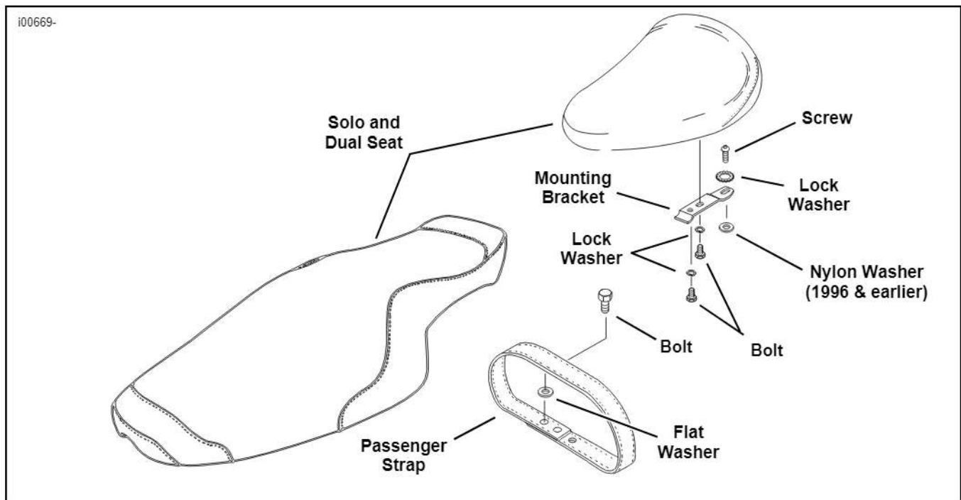
Figure 1. Original Stock Seat and Hardware
