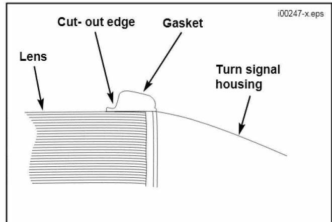
Figure 1. Gasket Location
