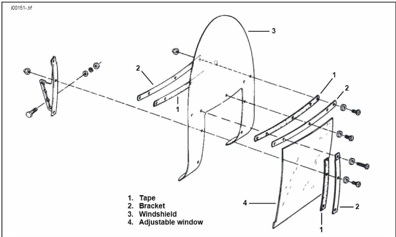
Illustration. Exploded View Of Windshield
