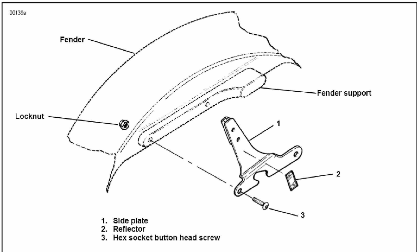
Figure 1. Side Plate and Hardware Installation
