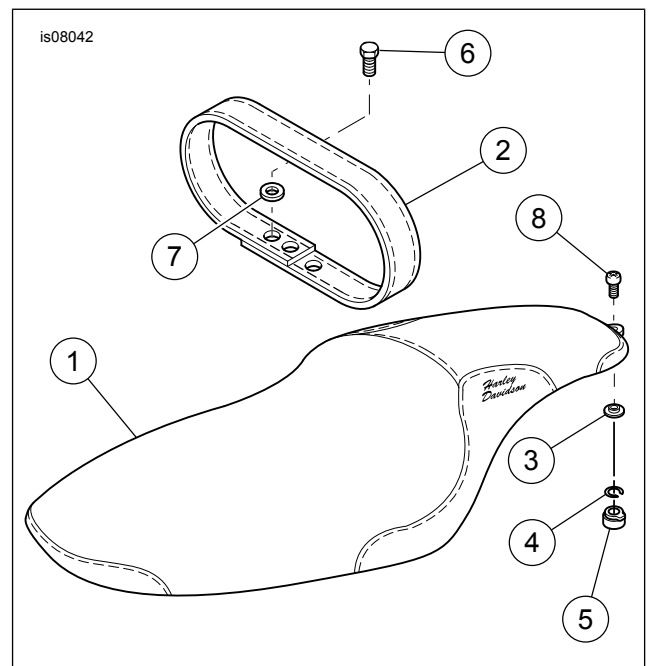
Figure 1. Service Parts
