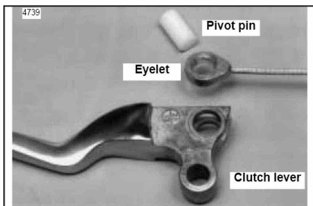
Figure 1. Cable Installation
