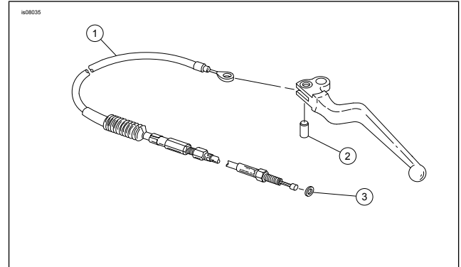
Figure 1. Service Parts
