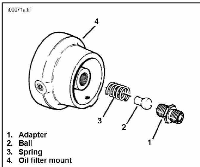
Figure 1. Oil Filter Adapter Assembly
