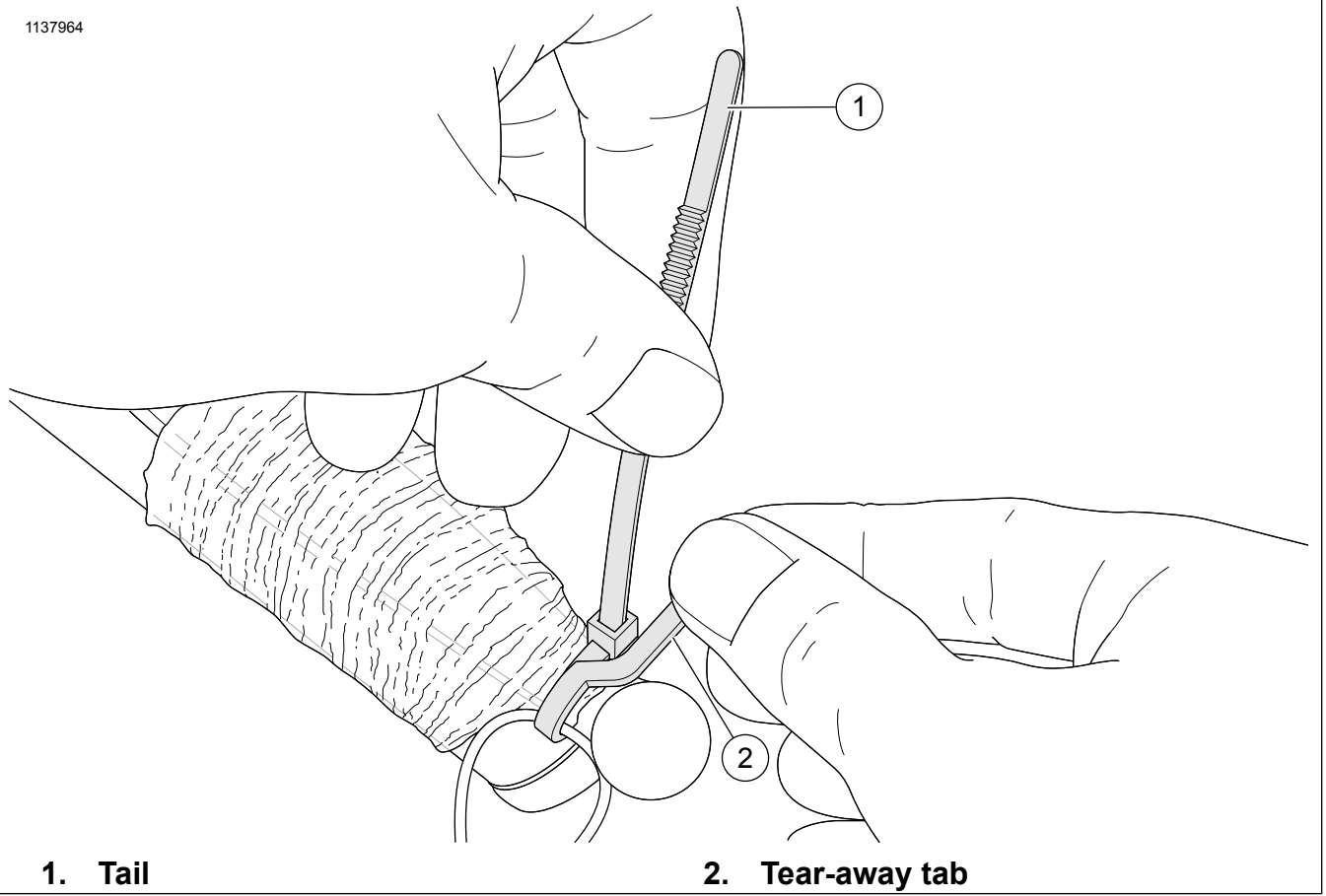
Figure 1. Tear-Away Cable Strap
