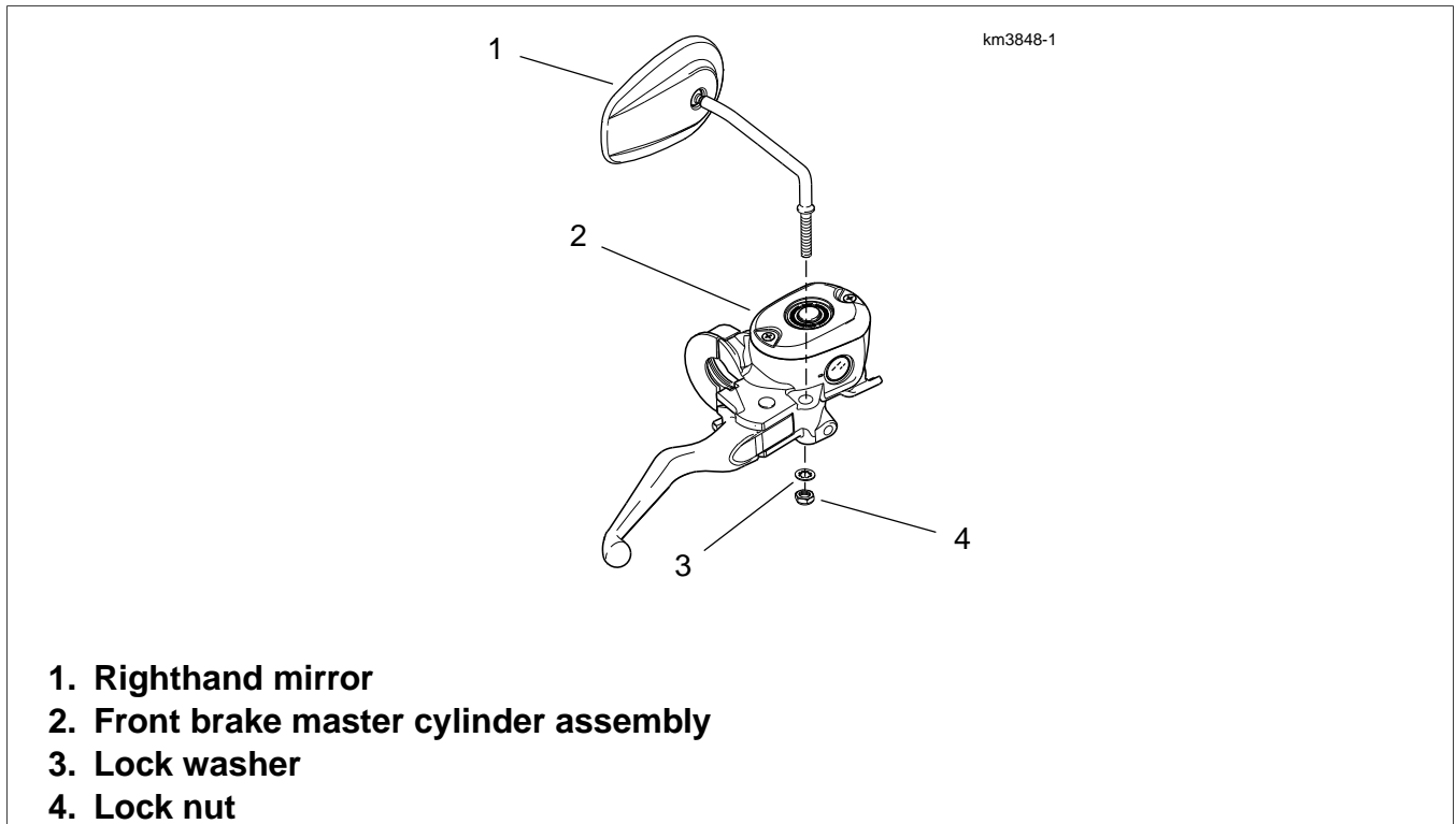
Figure 1. XL Mirror Stem (protective cap removed)
