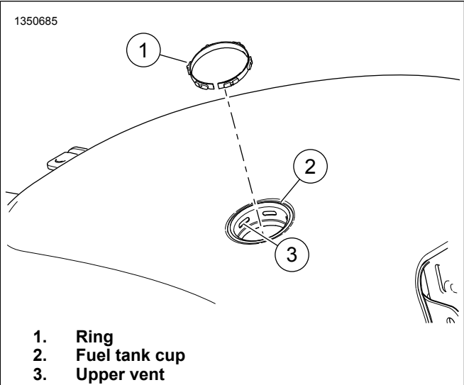
Figure 3. Previous Softail Fuel Tank
