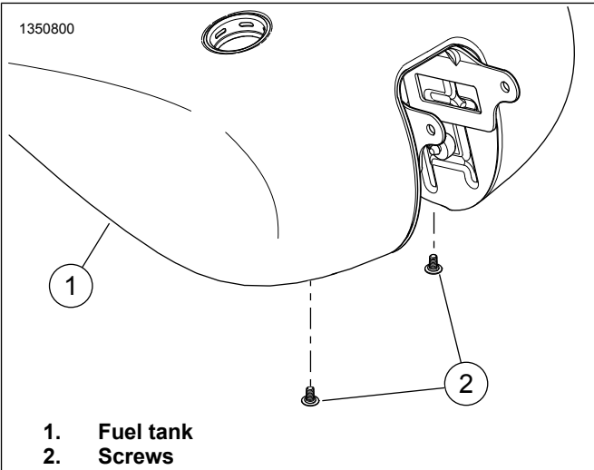
Figure 4. Fuel Tank - Screws (Typical)
