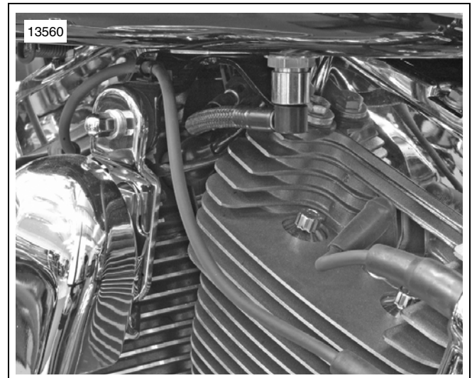
Figure 1. Correct Spark Plug Routing
