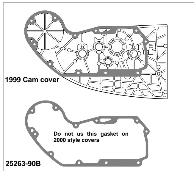
Figure 2. 1999 Cam cover and gasket
