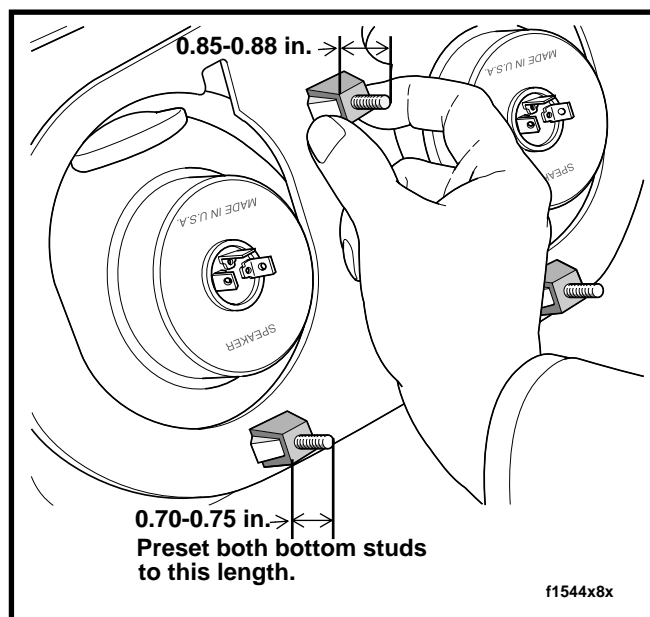
Figure 2. Presetting Adjuster Studs
