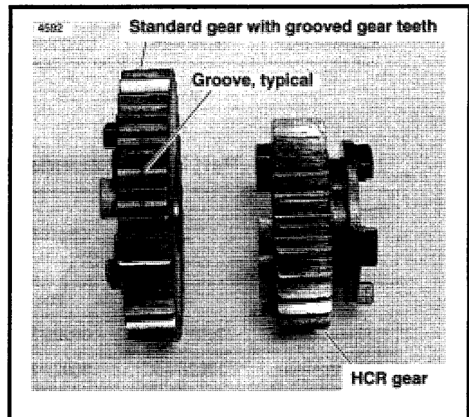
Figure. HCR And Standard Gears
