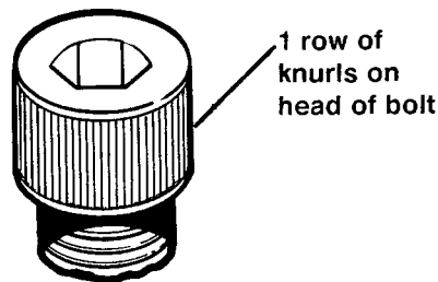
NEW REPLACEMENT BOLT (Part No. 855A)
