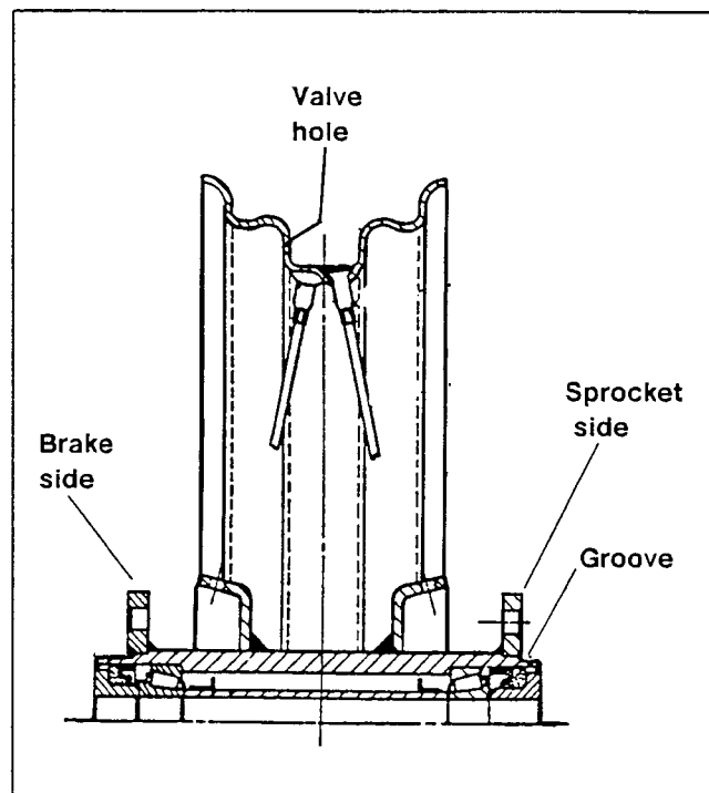
Wheel Assembly
