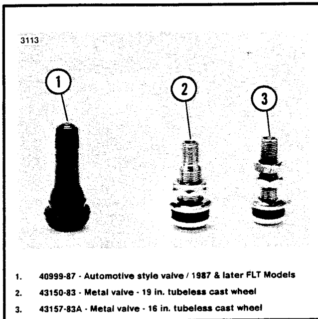
Figure 1. Tubeless Tire Valve Stem
