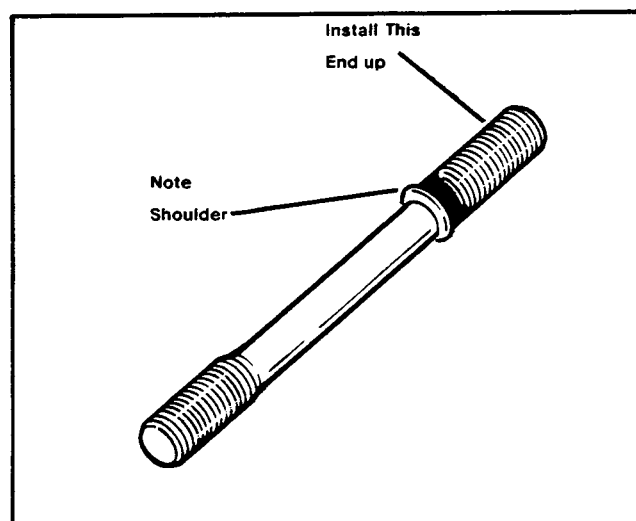
Figure 1. 1987 1/2 Cylinder Stud
