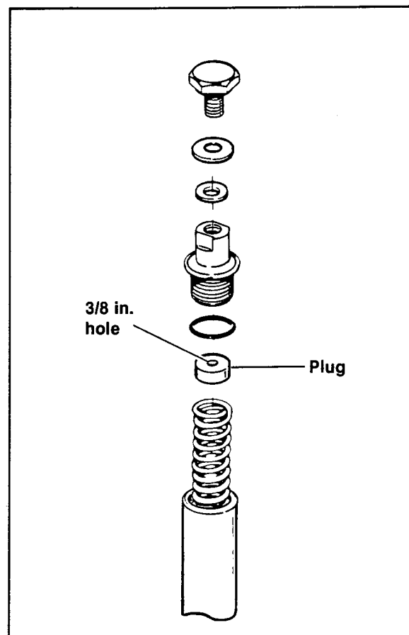
Figure 1. FLST Fork Tube Configuration Plug
