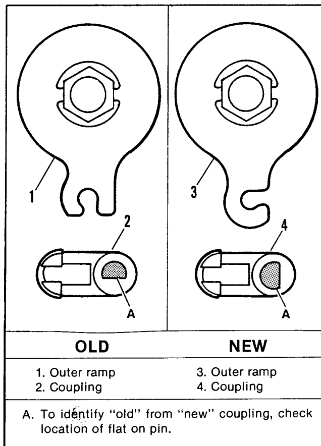
Figure 1. Clutch Release Components
