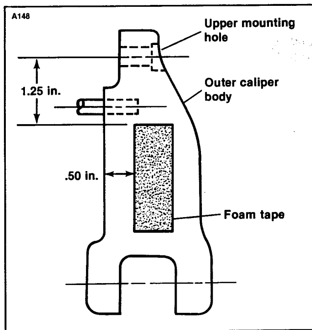
Figure 2. Foam Tape Installation — FLT Models
