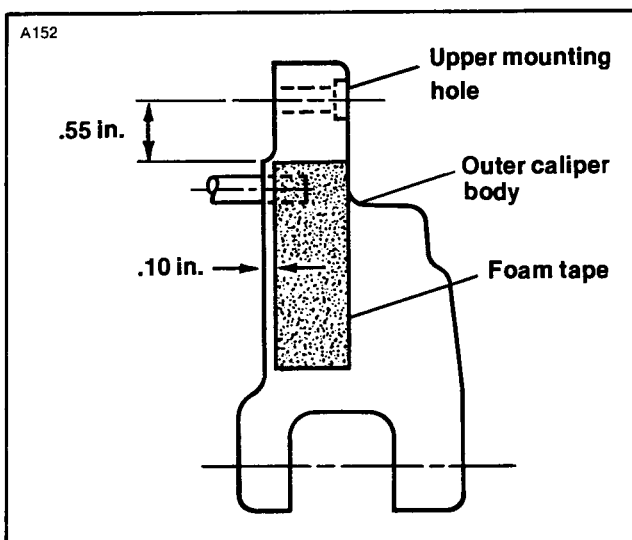
Figure 1. Foam Tape Installation — XL and FX Models
