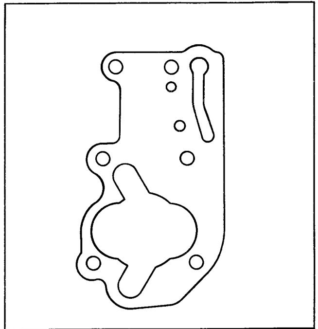
Figure 2. Incorrect Gasket, Part No. 26273-80 (Use with late 1980 oil pumps only.)
