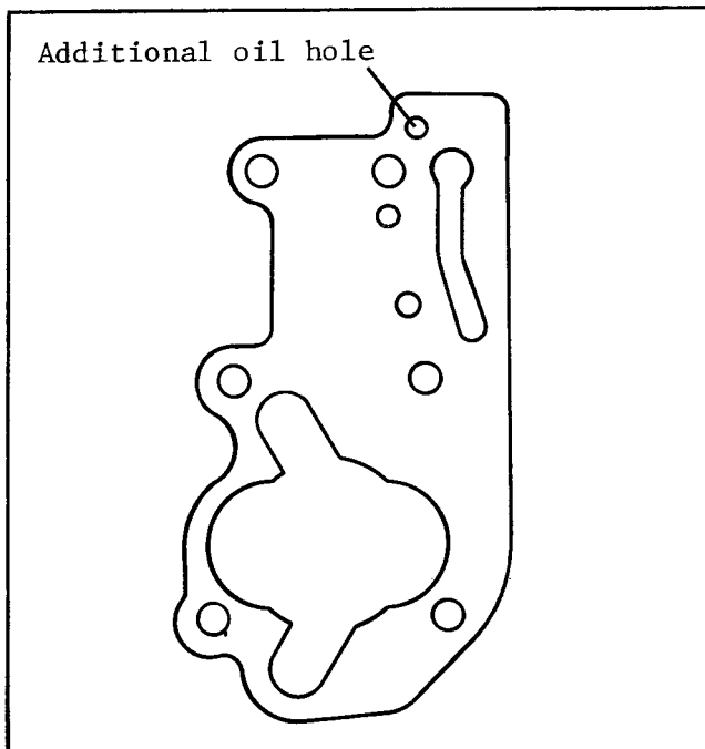
Figure 1 Correct Gasket, Part No. 26273-80A
