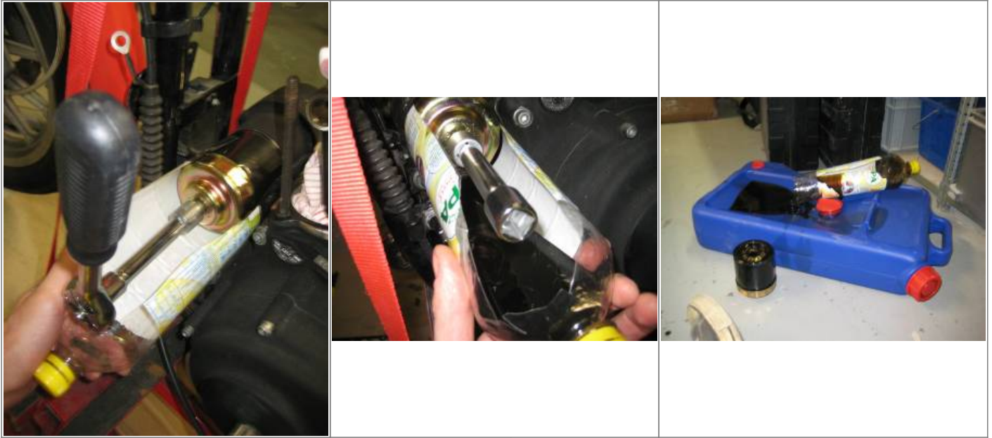
An old antifreeze jug with the side cut open making a drain pan and the cut piece is bent as a funnel. 21)
